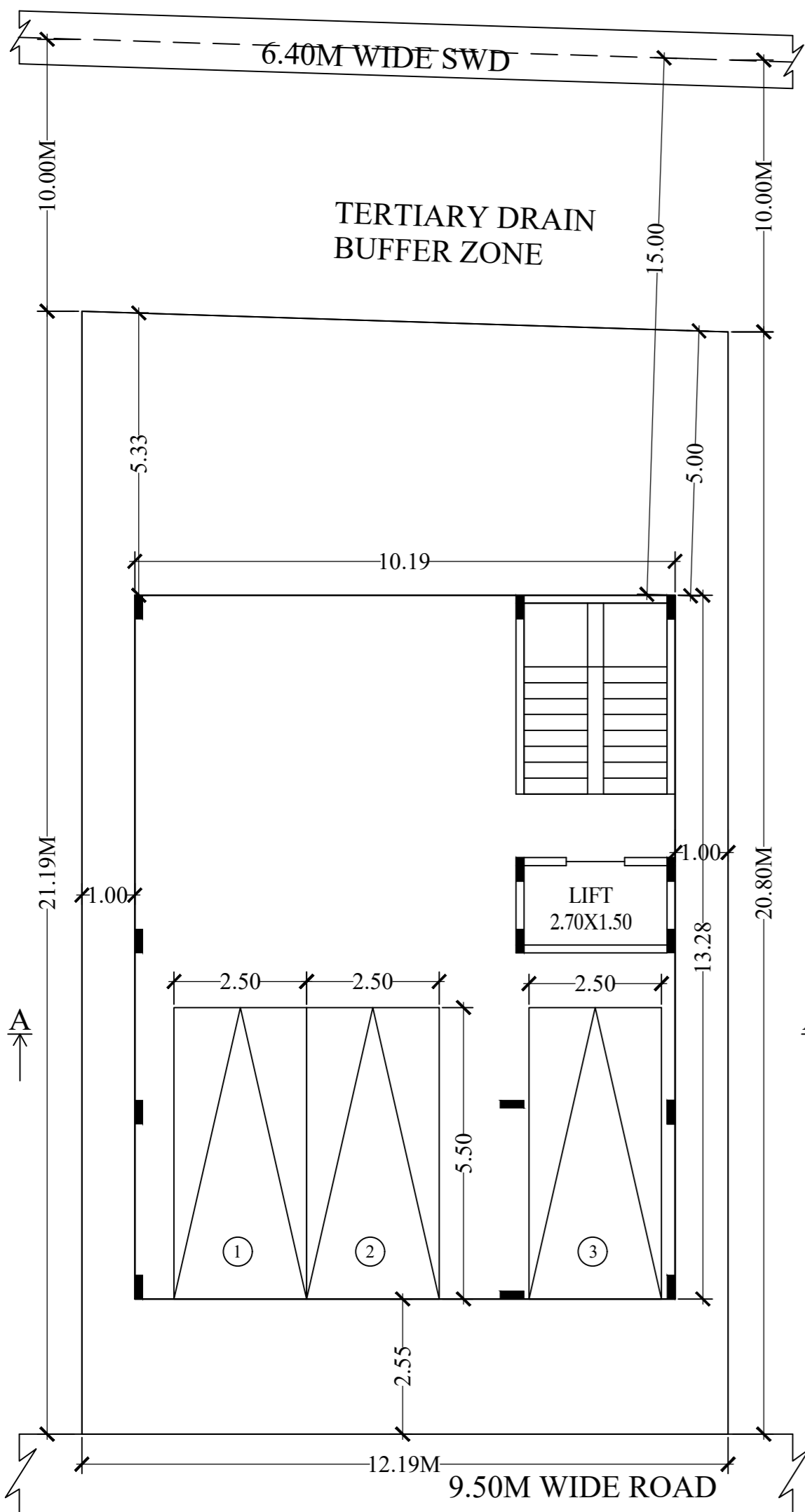
PROPOSED STILT FLOOR PLAN
